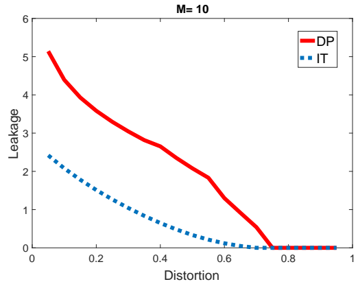
Fig. 7: Differential Privacy vs Information Theoretic Leakage for \mathcal{P}_{II}^{(10)} in Table II.
