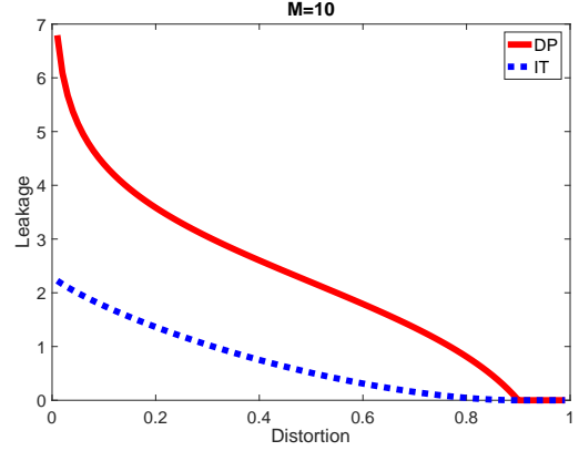
Fig. 6: Differential Privacy vs Information Theoretic Leakage for Class I source sets and M = 10 .
