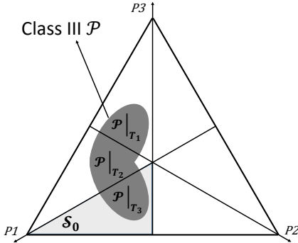
Fig. 2: A Class III source set \mathcal{P} .
